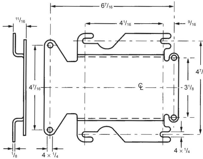
R410-7900 Mounting Bracket
