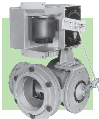
4" Adjustable Port Gas Valve Honeywell Electric Operator
