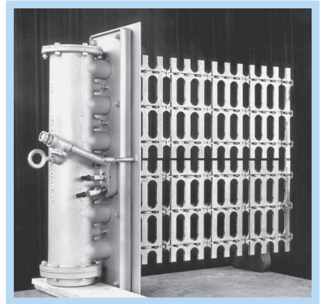
Fume incinerating flame grids use gas as the auxiliary fuel.
