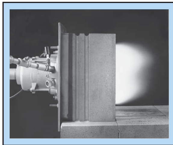
Figure 3. 4841-3-F Burner Flame--8" long with 12 psi air (298 000 Btu/hr). Optional flanged mounting ① shown.
