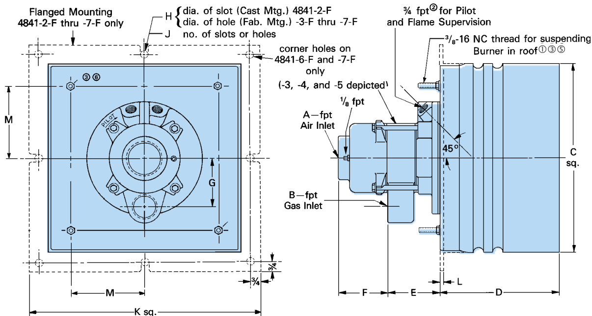
Figure 3. 4841-3-F Burner Flame--8" long with 12 psi air (298 000 Btu/hr). Optional flanged mounting ① shown.
